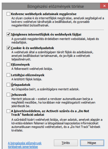
Internet Explorer
